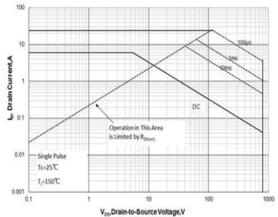
Fig 12 Safe Operation Area (ITO-220AB)
