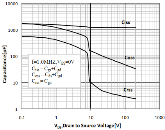
Fig 9 Capacitance Characteristics
