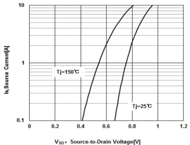
Fig 6 Body-Diode Characteristics
